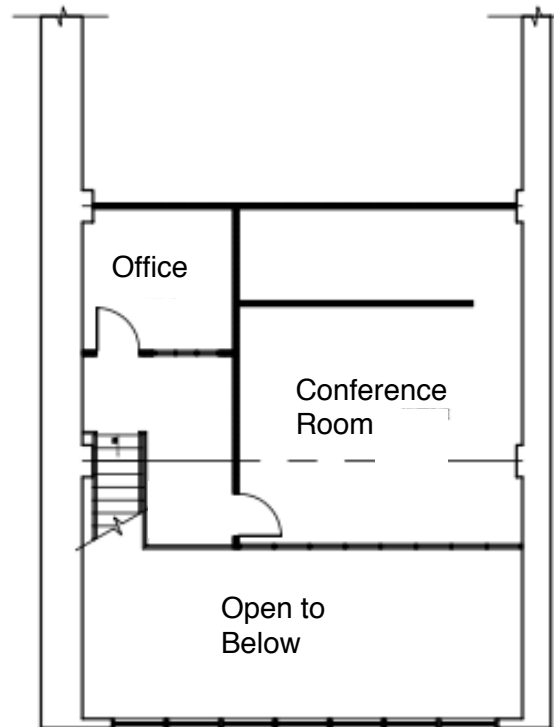
MEZZANINE PLAN
