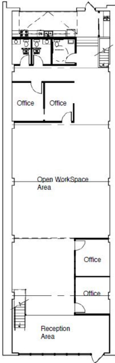
FIRST FLOOR PLAN 1/16" = 1'-0"
