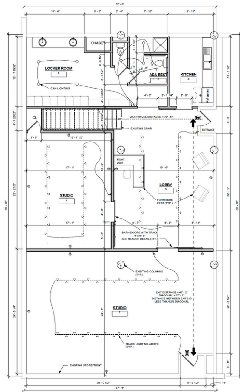
① MAIN FLOOR PLAN- NEW CONSTRUCTION 1/4" = 1'-0"
